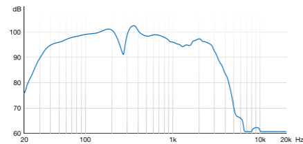
SENSITIVITY V-215B @ 2.83 V / m
