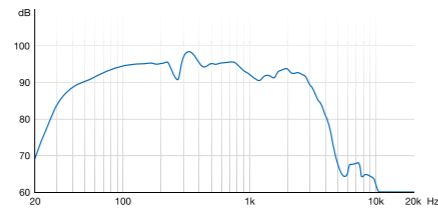
SENSITIVITY V-115B @ 2.83 V / m
